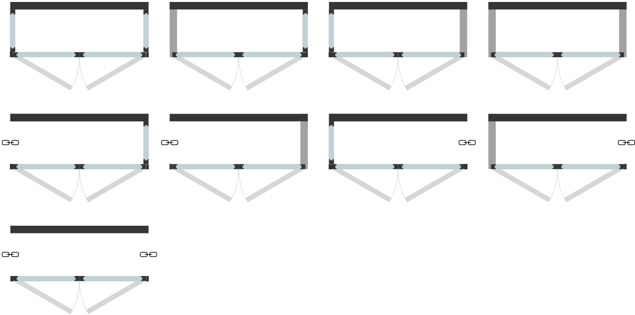
IsoCase modules can be joined to form a long wall section.
